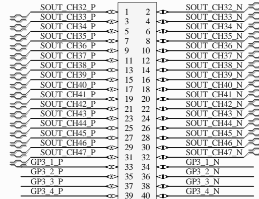
KEL8630E-040S-P_0.635mm
