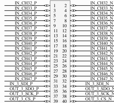
KEL8630E-040S-P_0.635mm SPLIT_OUTPUT3
