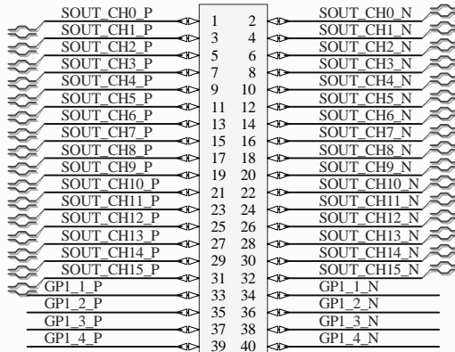
KEL8630E-040S-P_0.635mm
