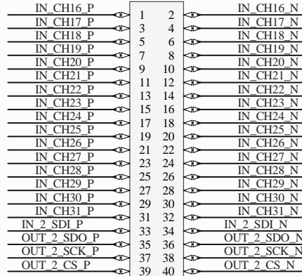
KEL8630E-040S-P_0.635mm SPLIT_OUTPUT2
