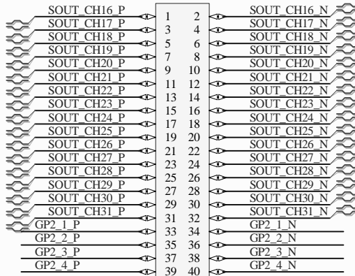
KEL8630E-040S-P_0.635mm
