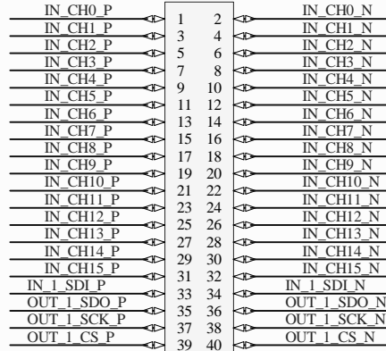
KEL8630E-040S-P_0.635mm SPLIT_OUTPUT1
